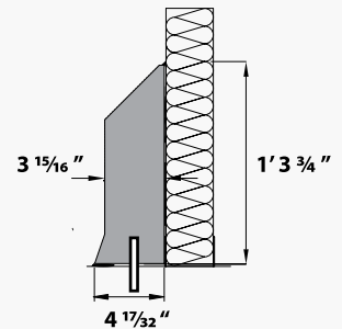
IP 30-40-50RB WITH REBATE OR R STRAIGHT
