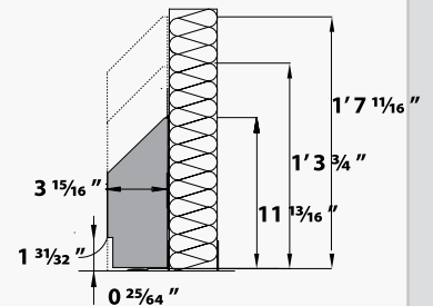
IP 30-40-50RB WITH REBATE OR R STRAIGHT
