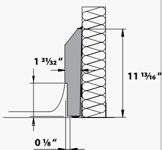
OP30RB CLEAN ROOM WITH REBATE
