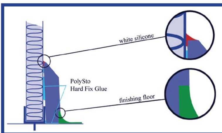
IP30,40,50RB (with rebate):
