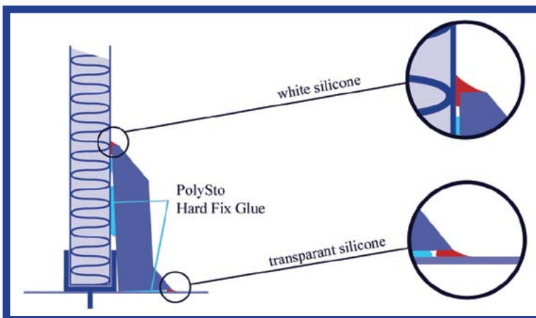
IP30,40,50R and IP40F and HPF (with feet):
