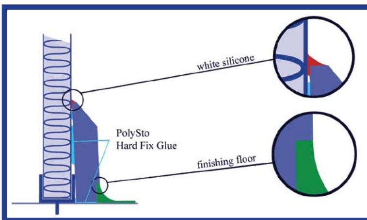
OP30RB (with rebate):
