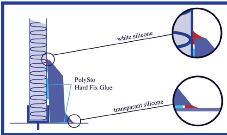
OP16F, OP20F & OP30F (with feet):
